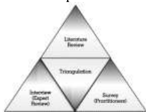
Gambar 1. Triangulasi Data
